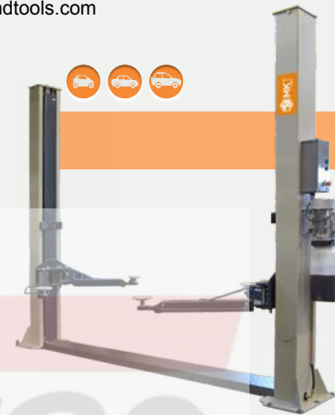
Hydraulic 2-Post Lift With Semi-Base 3500 Kg Manual unlocking
