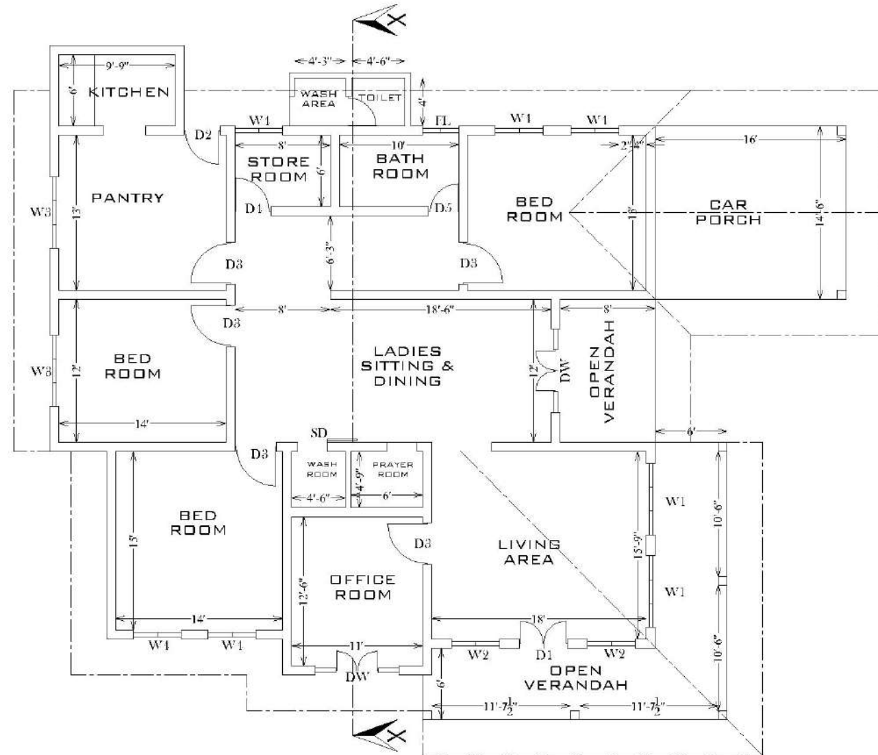
Floor Plan
